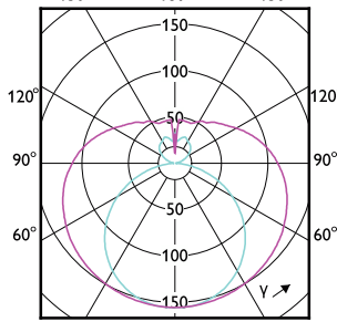
(cd/1000lm) 0° 150° 0-180° 180° 90-270° 150°
