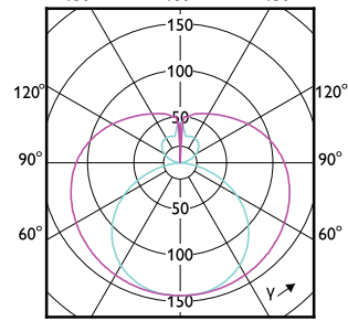
(cd/1000lm) 0° 150° 0-180° 180° 90-270° 150°
