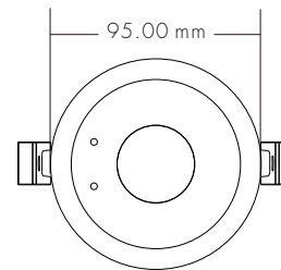
Ceiling (drill hole \varnothing 86mm)
