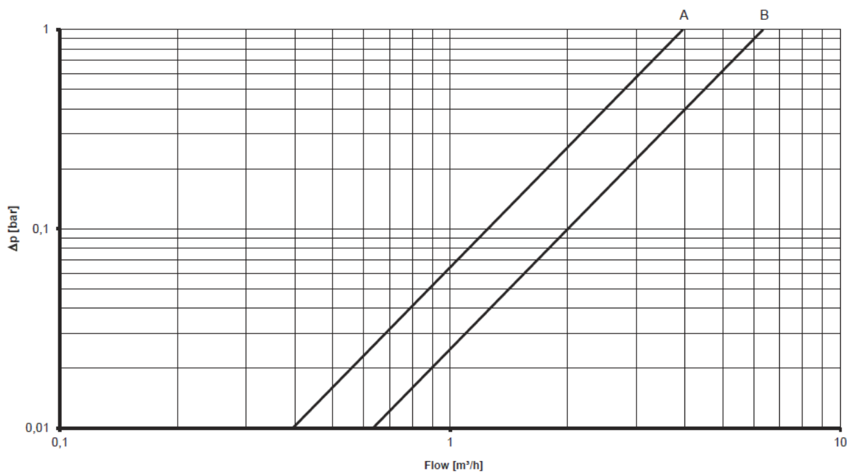
Tryktabs-diagram
