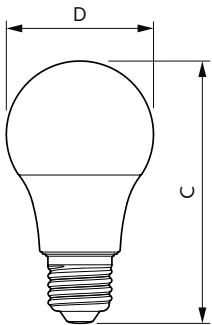
LEDbulb ND 8-60W A60 E27 827 2CT
