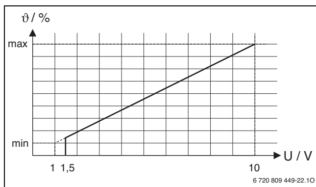
Fig. 2 Linear relationship between the 0-10 V signal ( U in volts) and required flow temperature \theta (in percent with reference to the maximum flow temperature)
