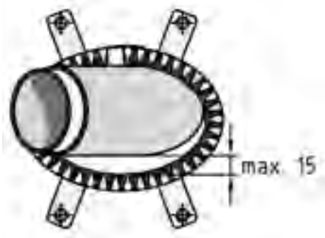
Fig. 46: Maximum allowable gap between pipe and fire protection collar
