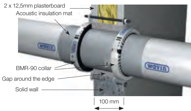
Fig. 51: Straight installation without sleeve / socket.
