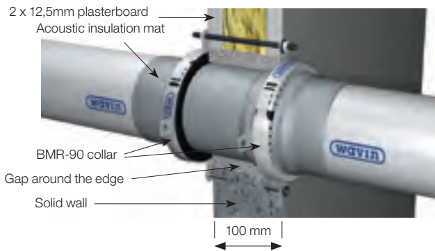
Fig. 50: Straight installation with sleeve / socket.
